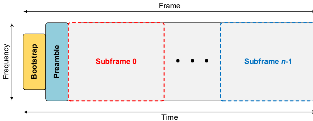
Figure 7.10 Frame structure.
