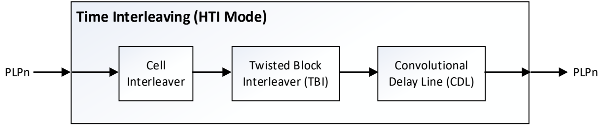
Figure 7.4 Block diagram for time interleaving for HTI mode.
