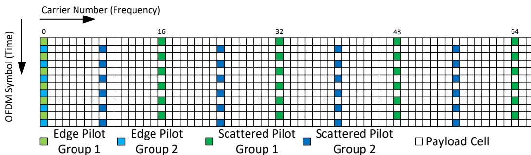
Figure L.9.7 MIMO pilot scheme MP8_2 for Walsh-Hadamard pilot encoding.
