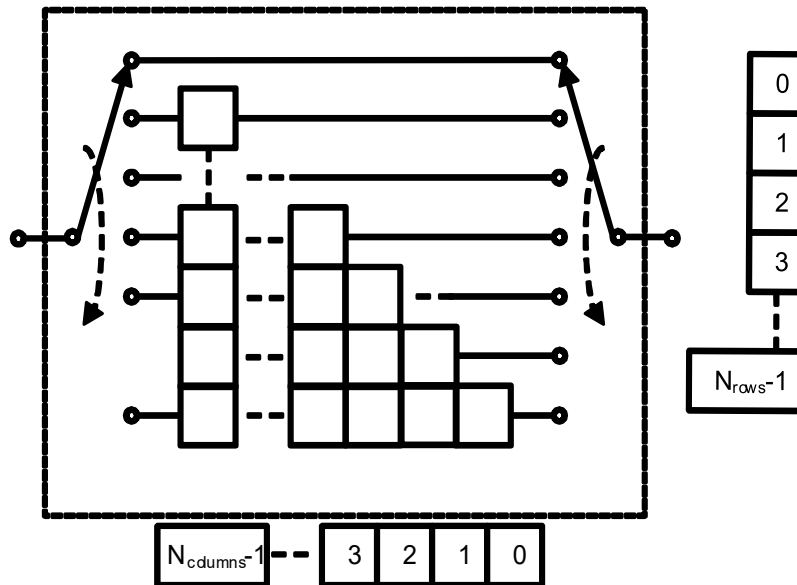
Figure 7.3 Block diagram of the Convolutional Time Interleaver.
